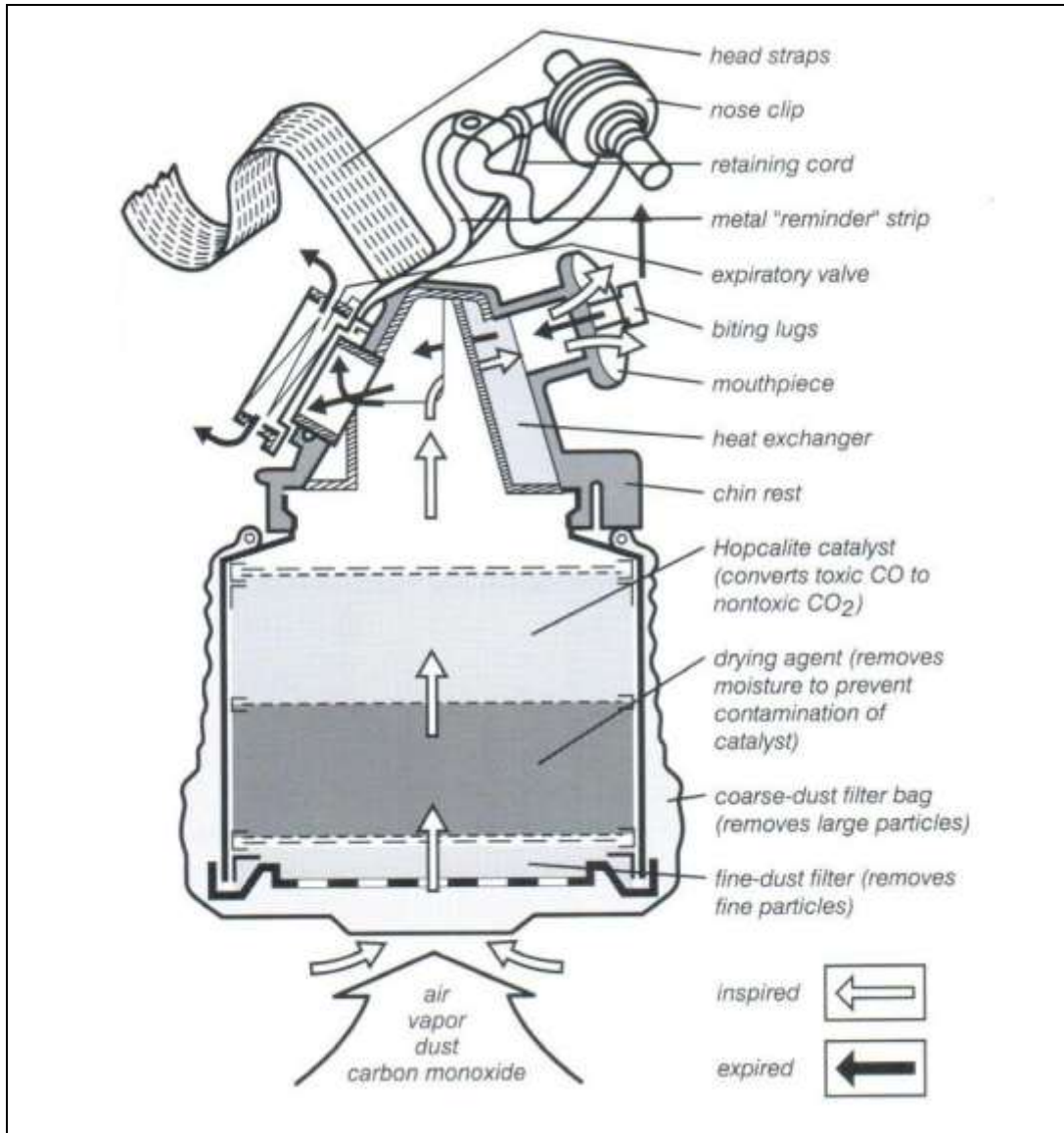
Fig 8-1: How a Self-Rescue functions
