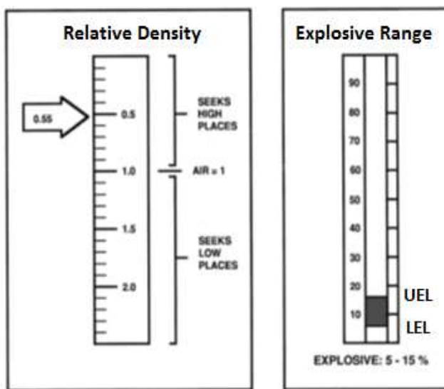
Fig 5.1 Relative density and Explosive range for Methane
