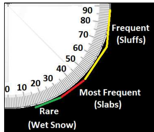
Fig 3.1 Slope steepness and avalanches
