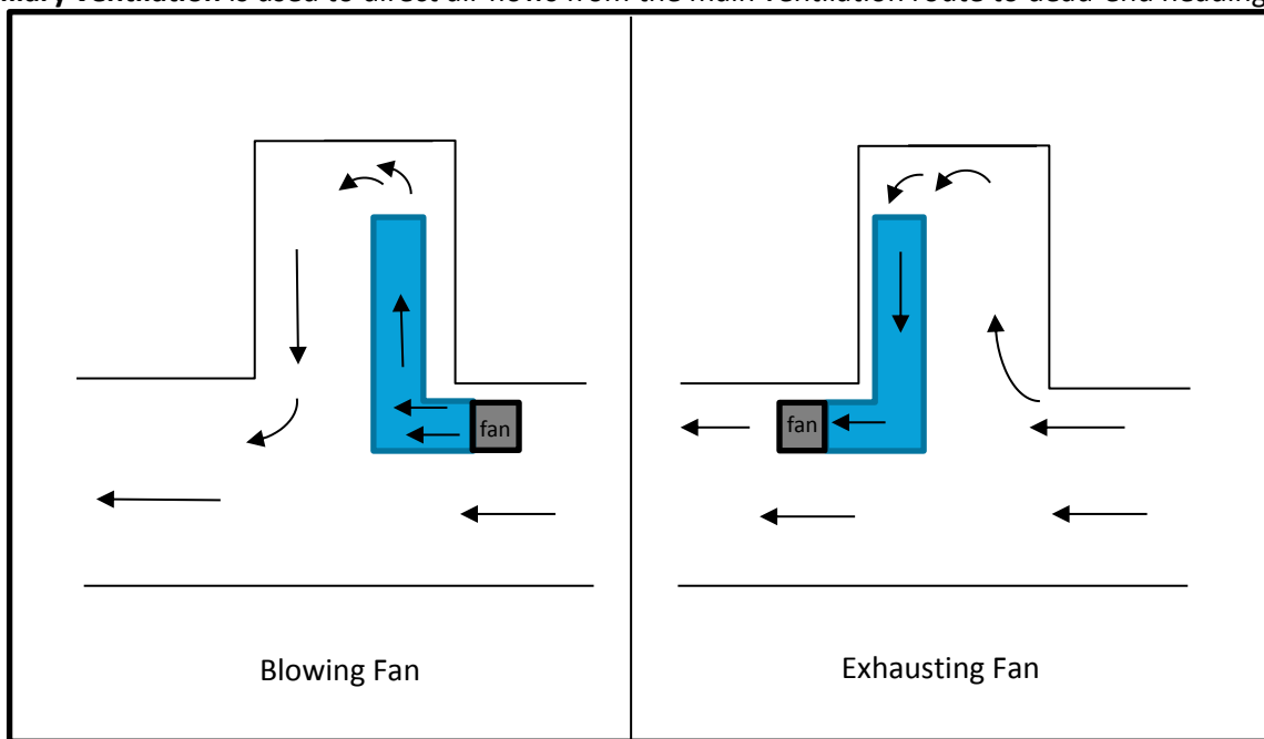
Fig 12.1: Blowing and Exhausting fans providing auxiliary ventilation
